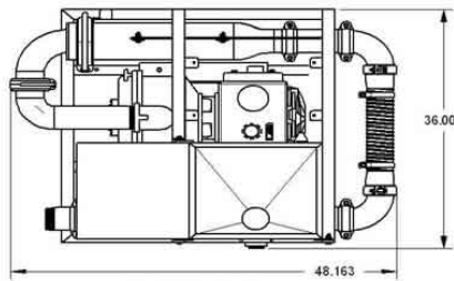
M3-G ( Gasoline ) DRY WEIGHT 525 lbs. Height 35 1/2" (Height 50" with optional gas tank)
